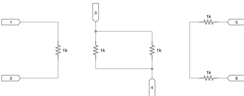
Electrical Schematic: Parallel & Series Circuit Comparisons
