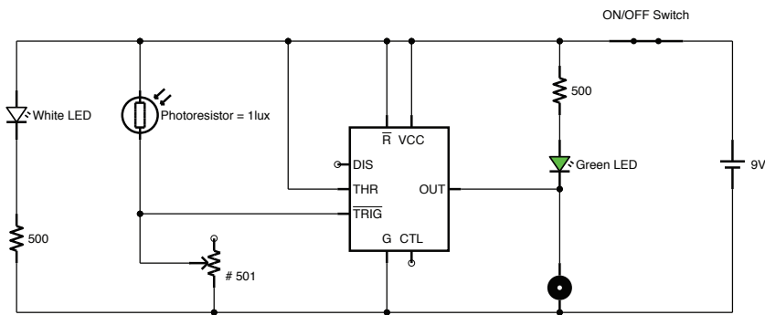
Electrical Schematics
